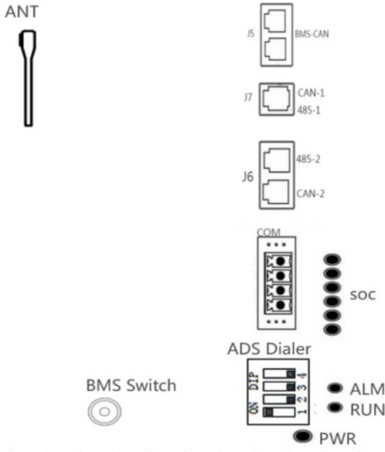
Fig. 5-2 Peration Panel
