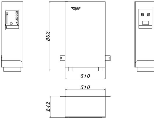
Fig. 5-1 Product Dimensions
